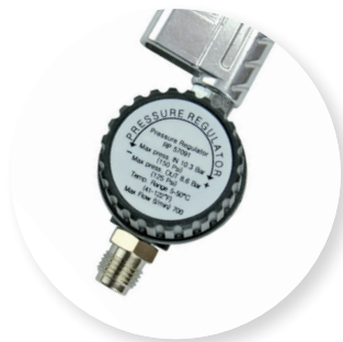
MICRO PRESSURE REGULATOR OPTIONAL (see item 4 on page 3)
